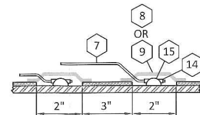
DETAIL 4 ATTACHING THE WIRES TO THE GAS MAIN SCALE: NO SCALE (CCV O-10) FIGURE 1
