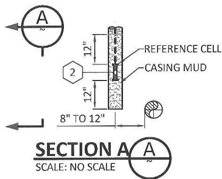
DETAIL 1 COUPON TEST STATION ABOVE GROUND SCALE: NO SCALE SHTS 10-23 CCV O-10.2
